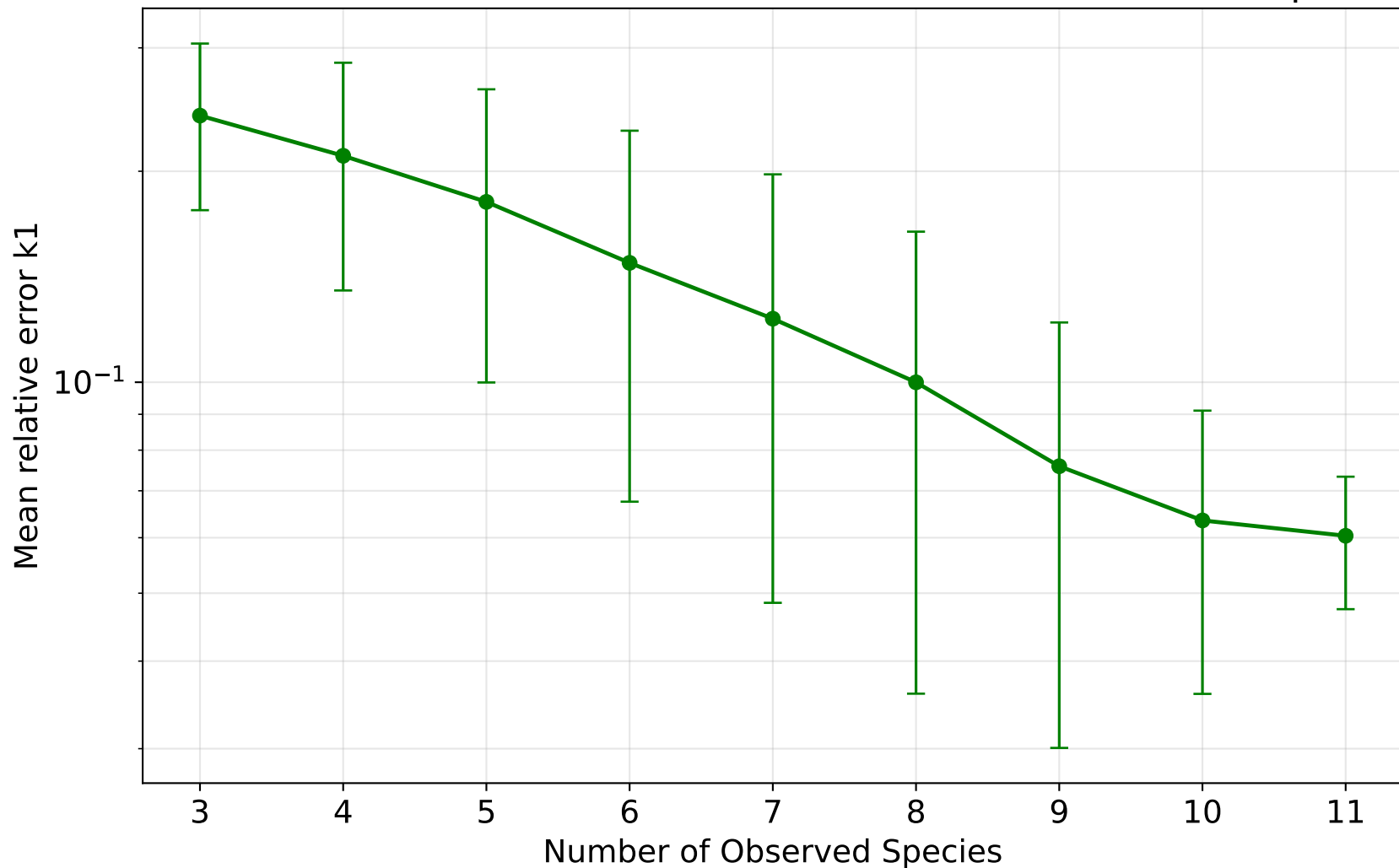
30, 30, 30 — Mean relative error k1 vs number of observed species
